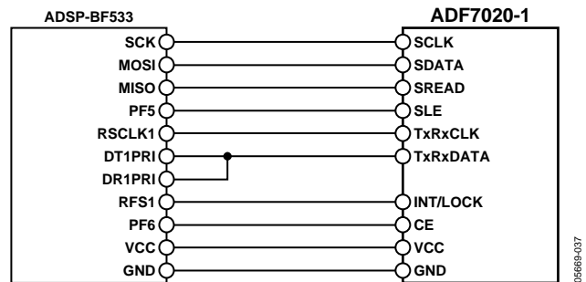
Figure 37. ADSP-BF533 to ADF7020-1 Connection Diagram
