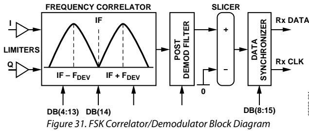
Figure 31. FSK Correlator/Demodulator Block Diagram
